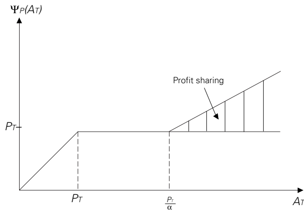
Figure 1. The payoff \psi_P(A_T) to the policyholder given no premature liquidation
