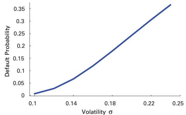
Figure 2. Probability with respect to volatility \sigma
