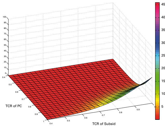
Figure 3. Probability of Default of PC for Stop Loss Guarantees [in %]
