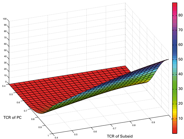
Figure 7. Probability of Default of PC for Quota Share Guarantees [in %]
