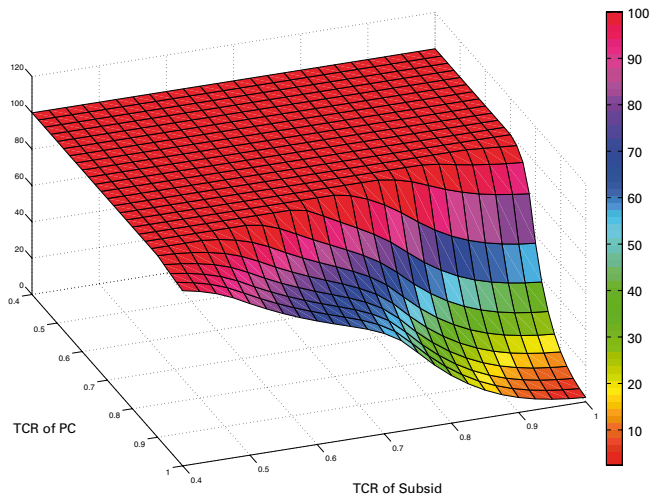
Figure 1. Realisable RDE in % fully consolidated RDE (12.4%) for Stop Loss under ES
