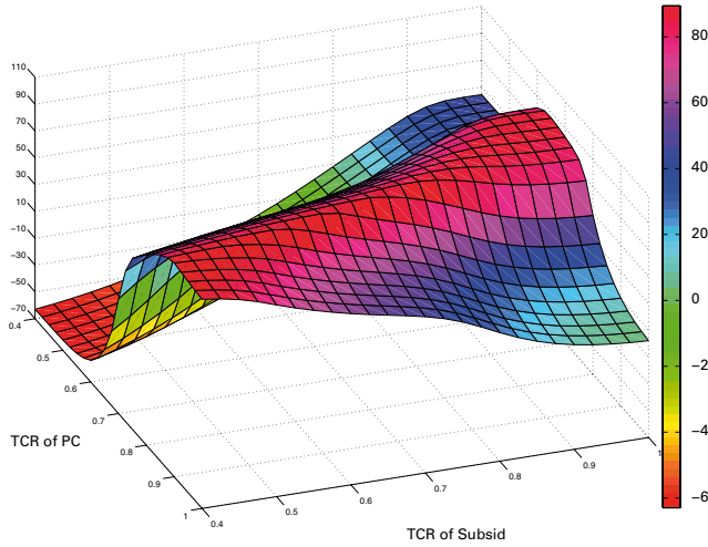
Figure 5. Realisable RDE in % fully consolidated RDE (12.4%) for Quota Share under ES
