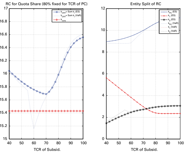
Figure 8. RC for Quota Share and Entity Split of RC
