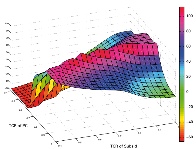
Figure 6. Realisable RDE in % fully consolidated RDE (12.4%) for Quota Share under VaR
