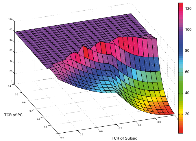
Figure 2. Realisable RDE in % fully consolidated RDE (12.4%) for Stop Loss under VaR
