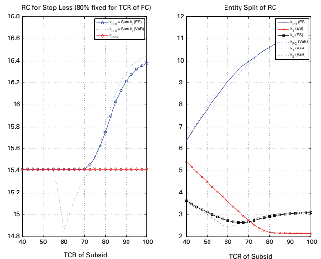
Figure 4. RC for Stop Loss and Entity Split of RC
